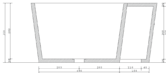
Cut 1-1
